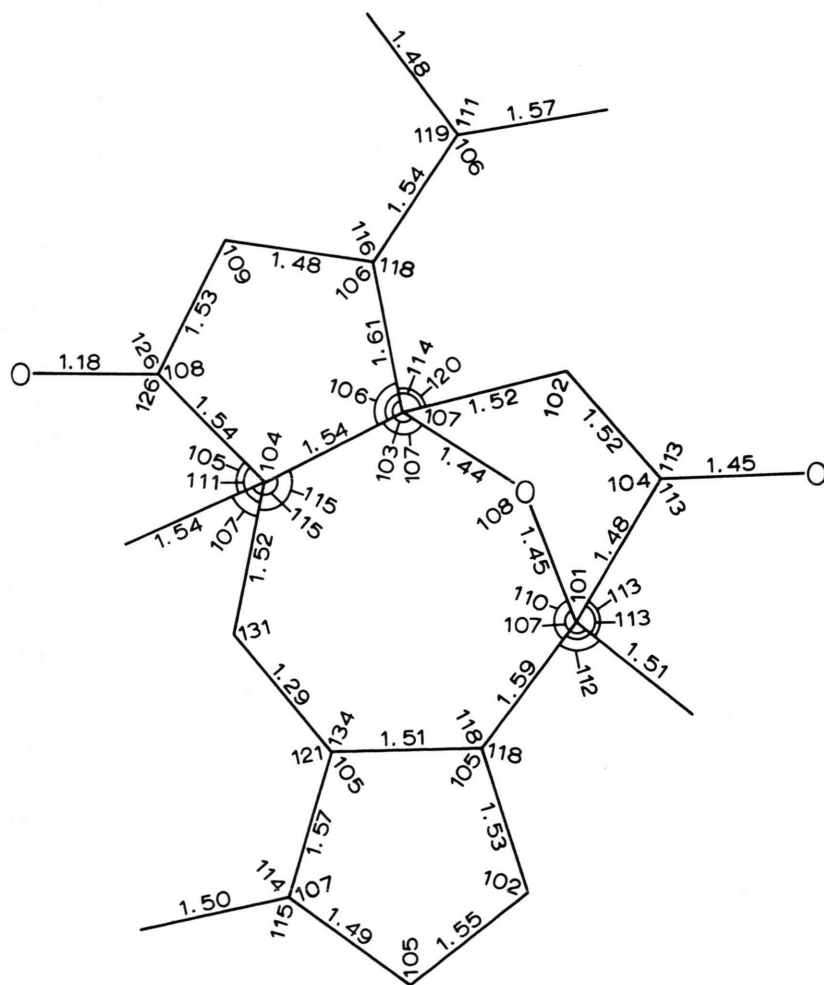
Fig. 2. Bond lengths and bond angles for 1 e.s.d.'s: \sigma_r=0.01 Å, \sigma_\alpha=1^\circ .
